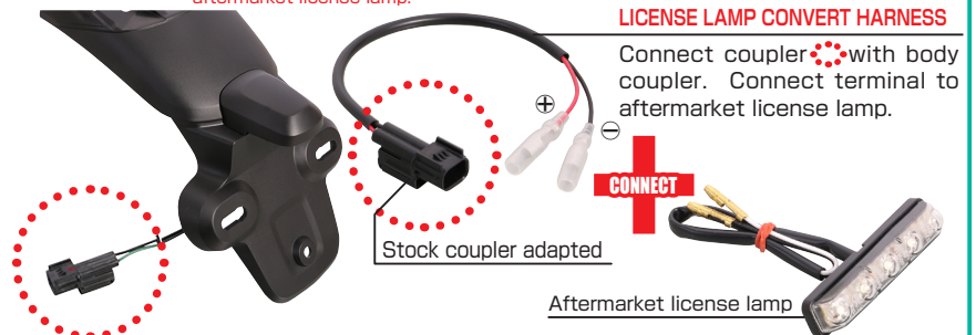
Joint harness to connect stock coupler with aftermarket license lamp.
