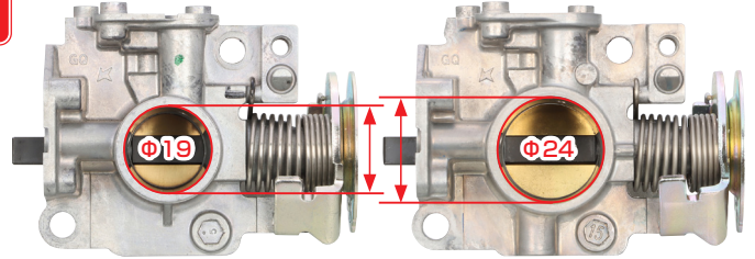
φ19 THROTTLE BODY (STOCK)
