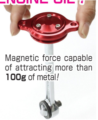
MAGNET IS INSTALLED IN THE FILTER COVER (REMOVABLE)
