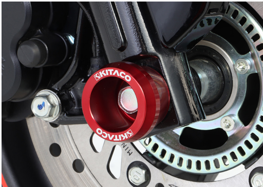
A machined aluminum axle protector for stock axle shafts and Kitaco hollow axle shafts. By allowing the vehicle to slide during a fall, damage is minimized.
