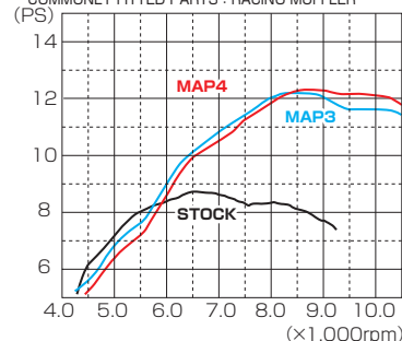
HIGH COMP PISTON 125cc COMMONLY FITTED PARTS : RACING MUFFLER (PS)
