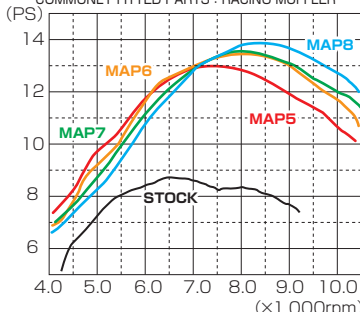
LIGHT 164cc COMMONLY FITTED PARTS : RACING MUFFLER (PS)
