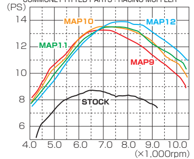
LIGHT 181cc COMMONLY FITTED PARTS : RACING MUFFLER (PS)
